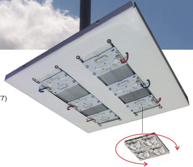
Rotatable Optics
